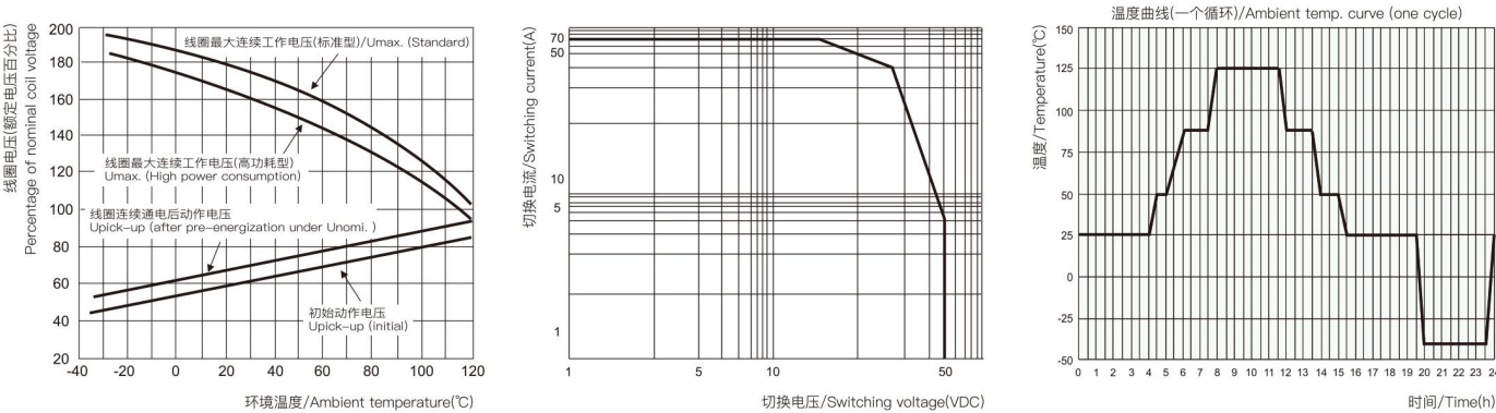
线圈连续通电电压范围 Coil operating voltage range
